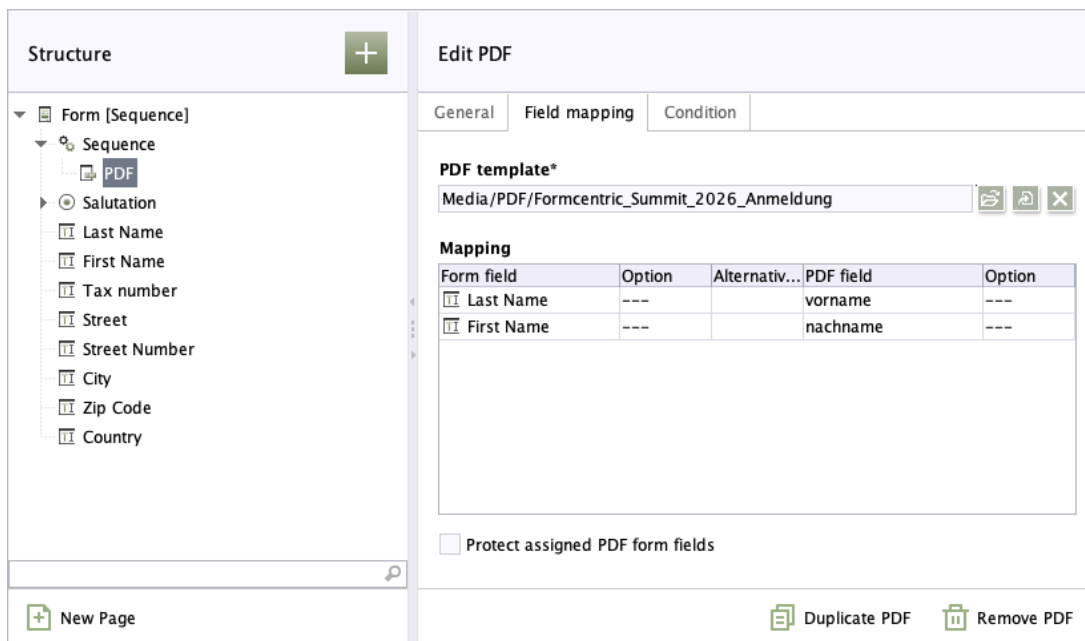
Figure 2.38. PDF
