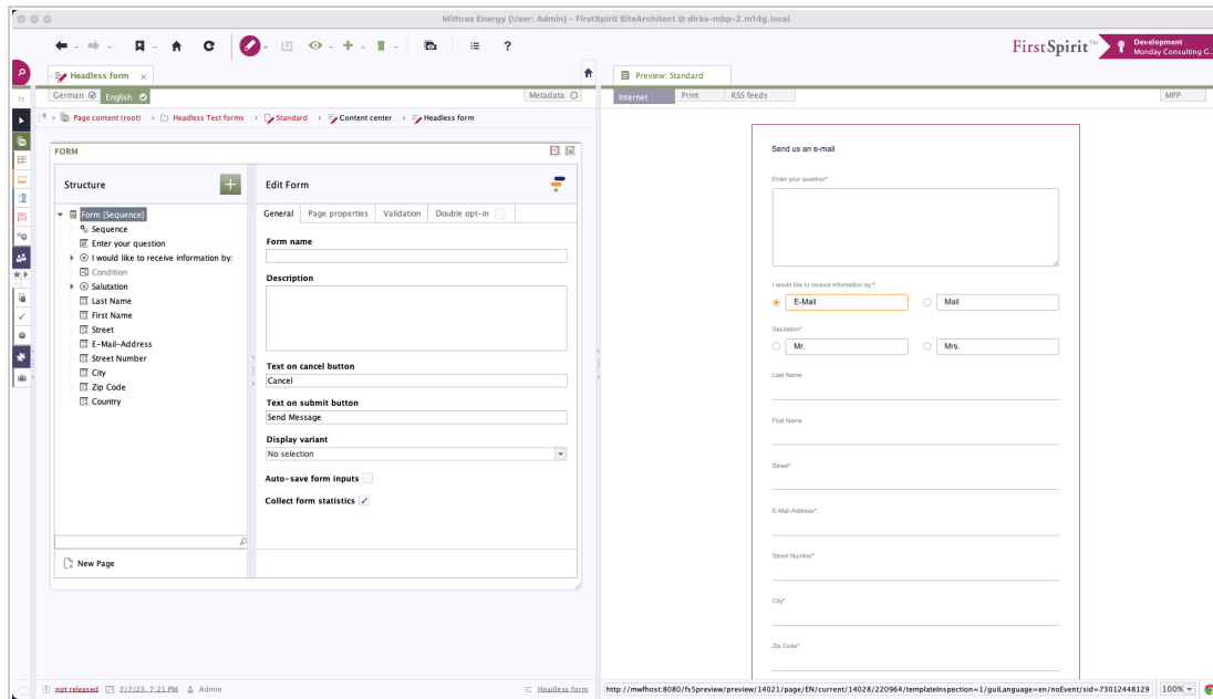
Figure 2.3. SiteArchitect preview
