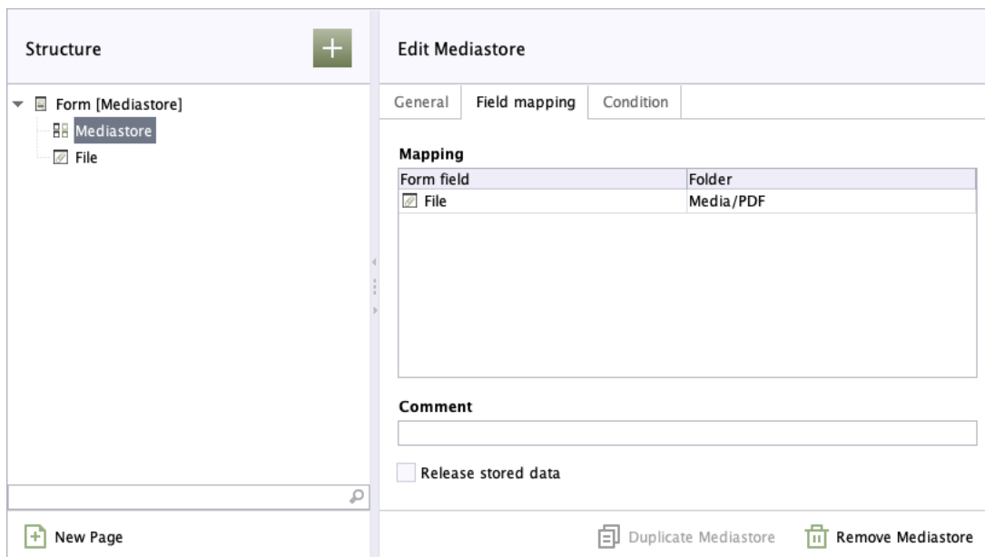
Figure 2.40. Media Management
