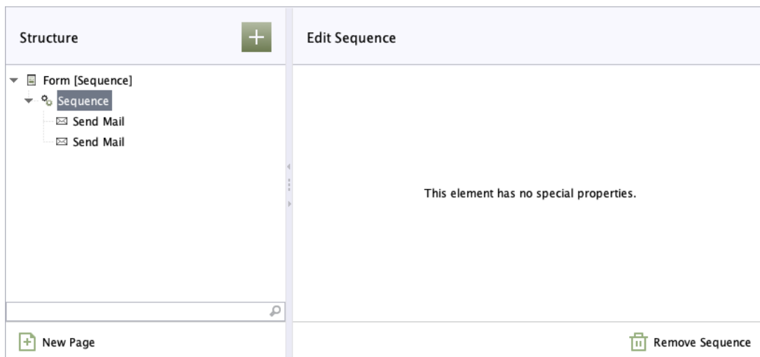
Figure 2.44. Sequence
