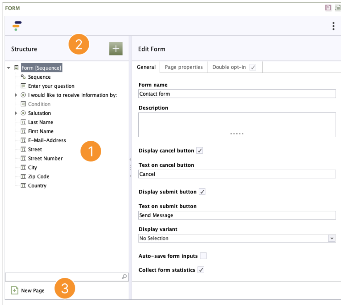
Figure 2.1. Editing interface
