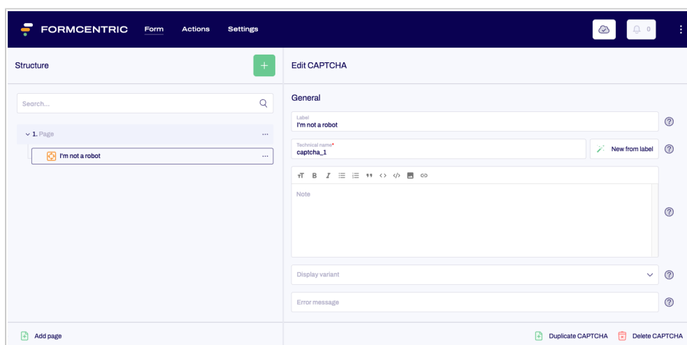
Figure 4.26. CAPTCHA
